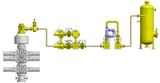
Land Drilling (LD)
