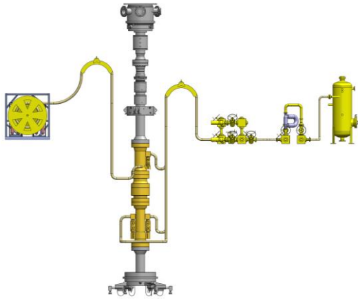
Below Tension Ring (BTR)
