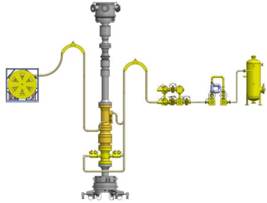
Above Tension Ring (ATR)
